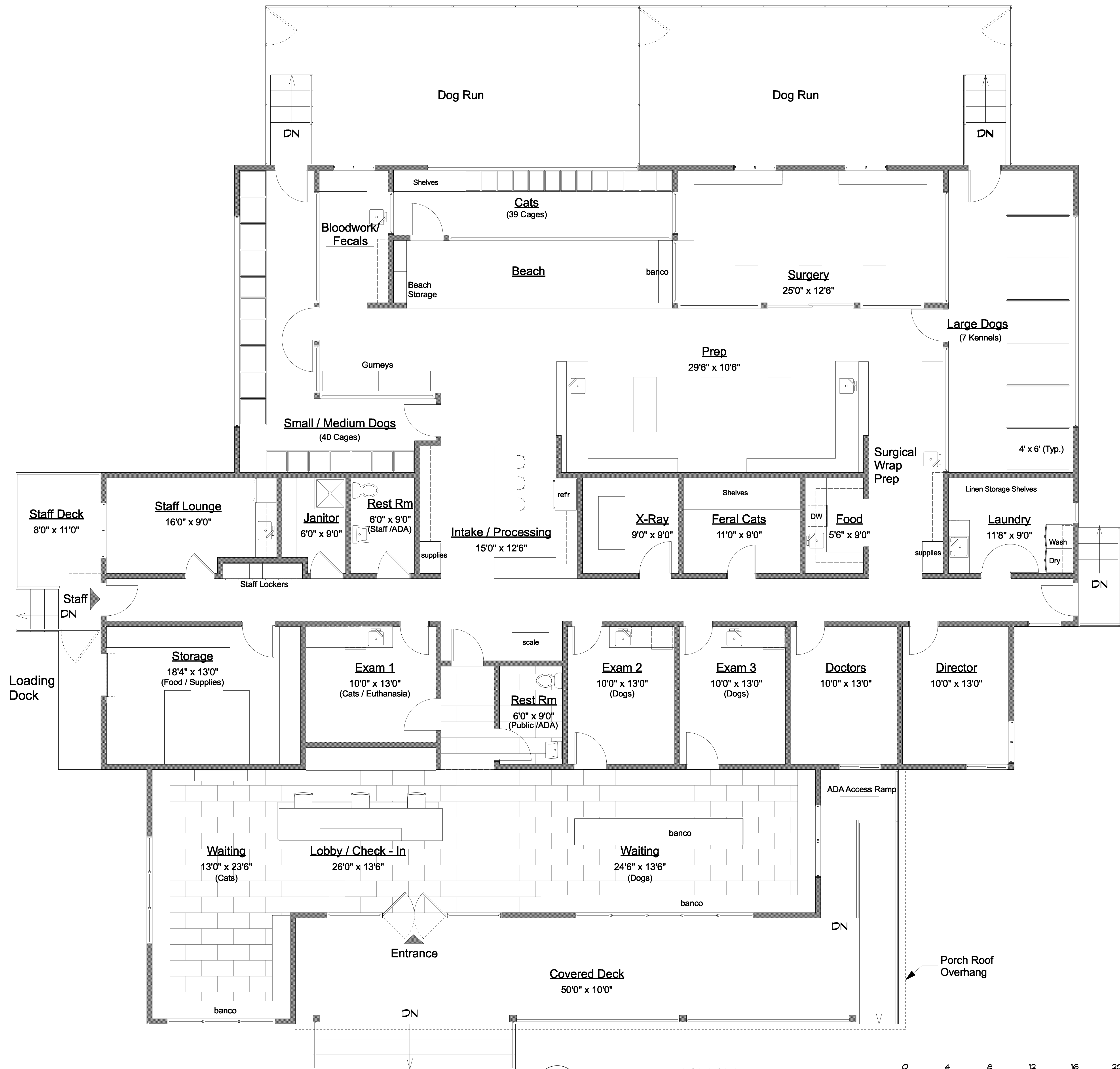
1 Floor Plan 9/20/23 5,836 sq.ft.
